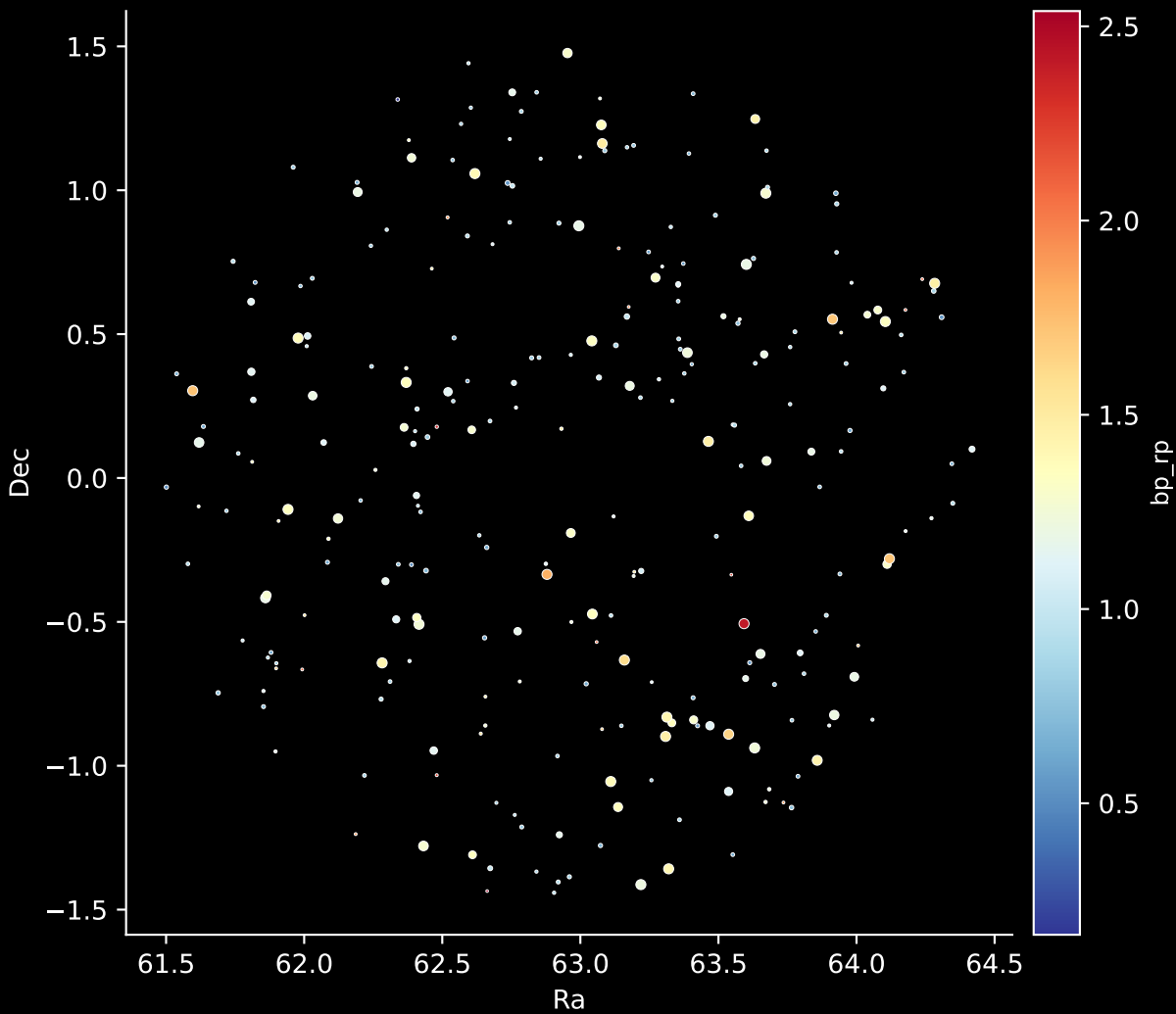
APOGEE DR17 Field: [054-35_MGA] Stars: 270
