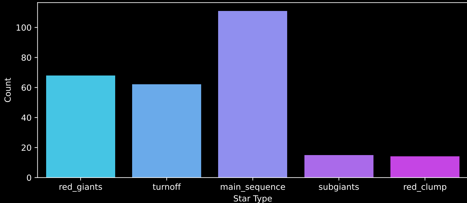
APOGEE DR17 Field: [054-35_MGA] Count plot of Star Type
