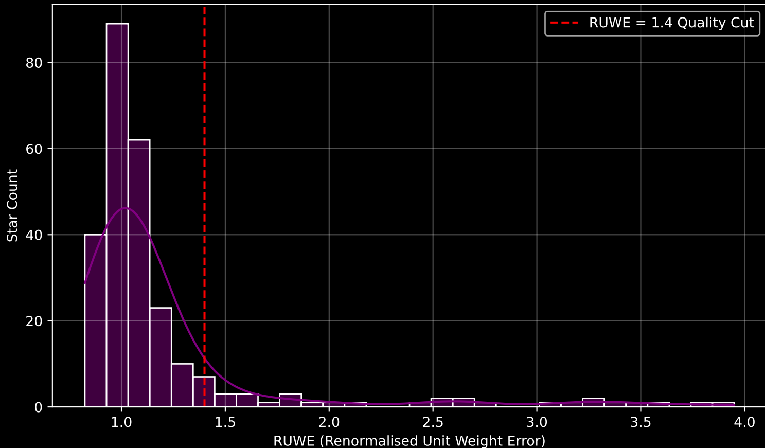
GAPOGEE DR17 Field [054-35_MGA] RUWE Distribution (n= 259)
