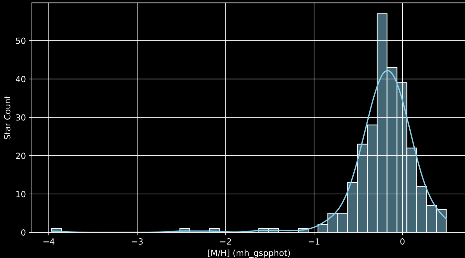
APOGEE DR17 Field: [054-35_MGA [M/H] (mh_gspphot) (n= 268)
