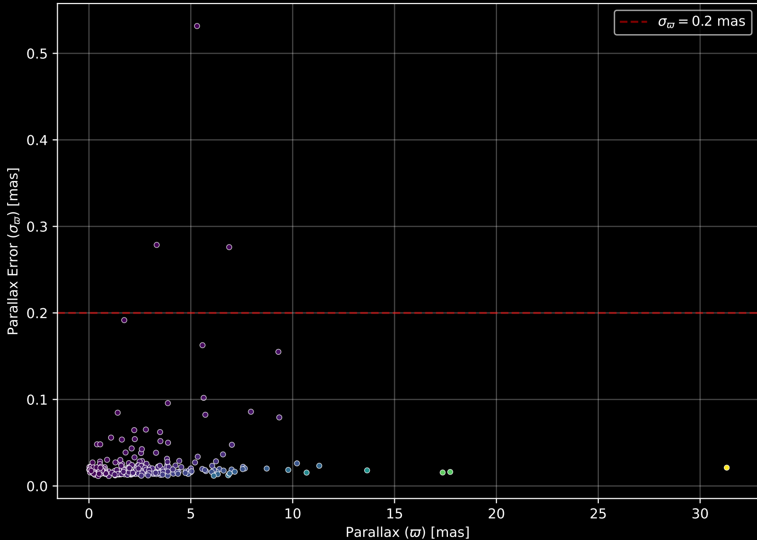
APOGEE DR17 Field: [054-35_MGA] Parallax Quality (n= 270)
