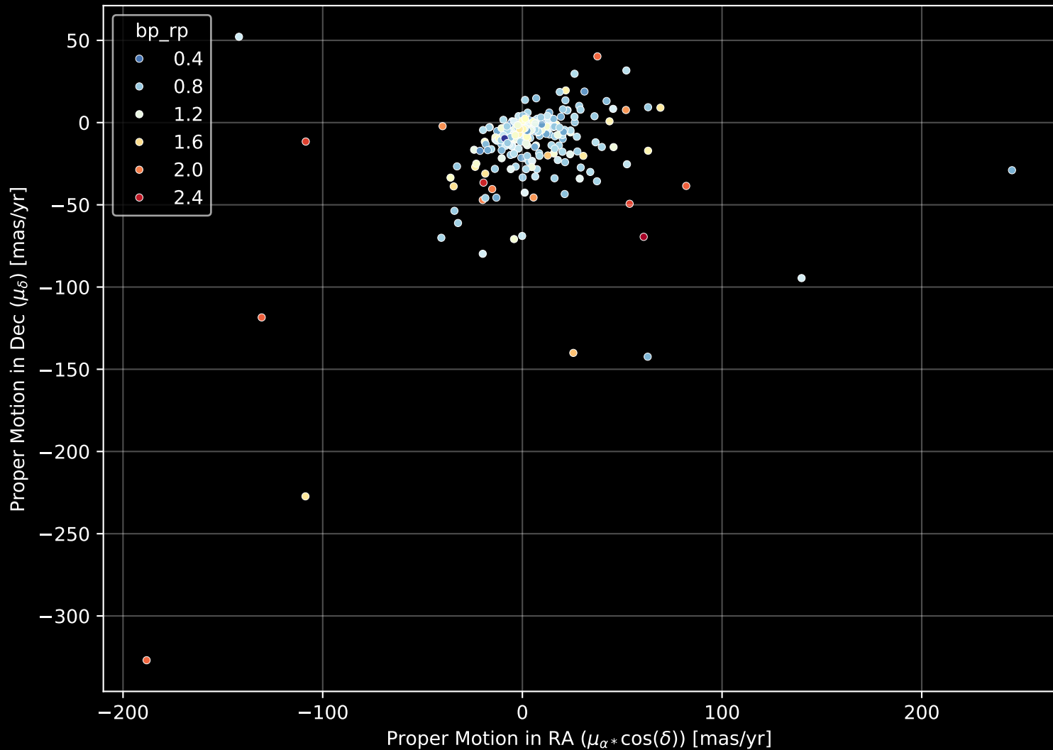
APOGEE DR17 Field: [054-35_MGA] Proper Motion Diagram (n= 270)
